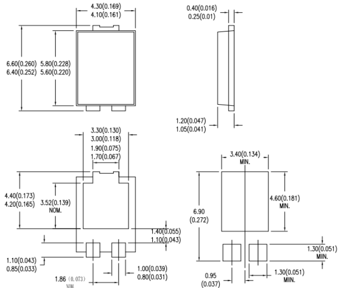
TO-277B
